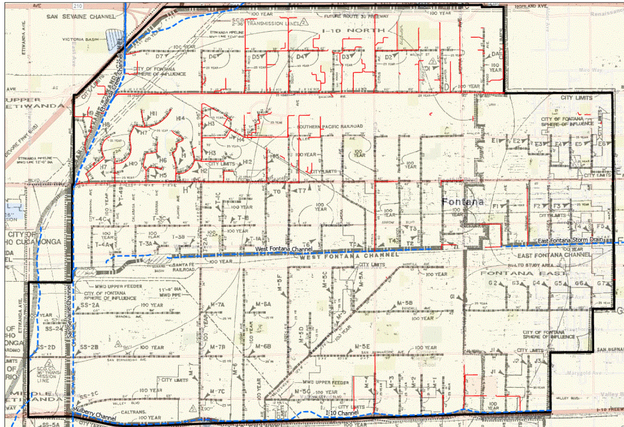
Figure 2-4. Comparison of Proposed Lines From the 1992 Master Plan to Existing Pipes in AOS 1 (red lines)
