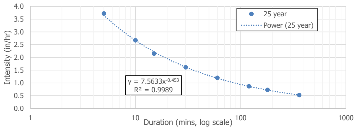
Figure 3-5. Intensity-Duration Curve for AOS 1 to Determine Runoff Coefficients for the Collector Hydrologic Analysis
