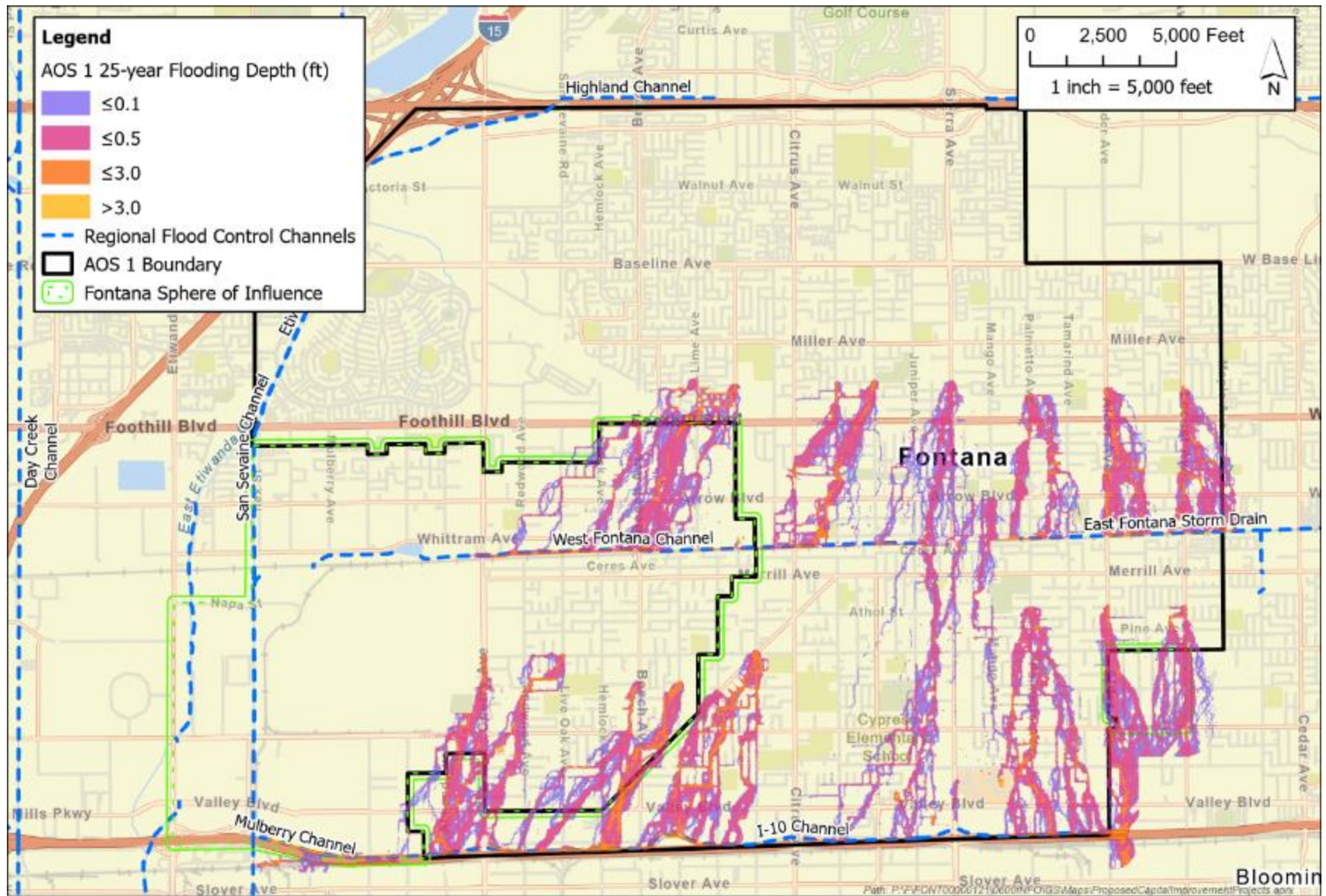
Figure 3-13. Existing Conditions 25-year Flooding in AOS 1
