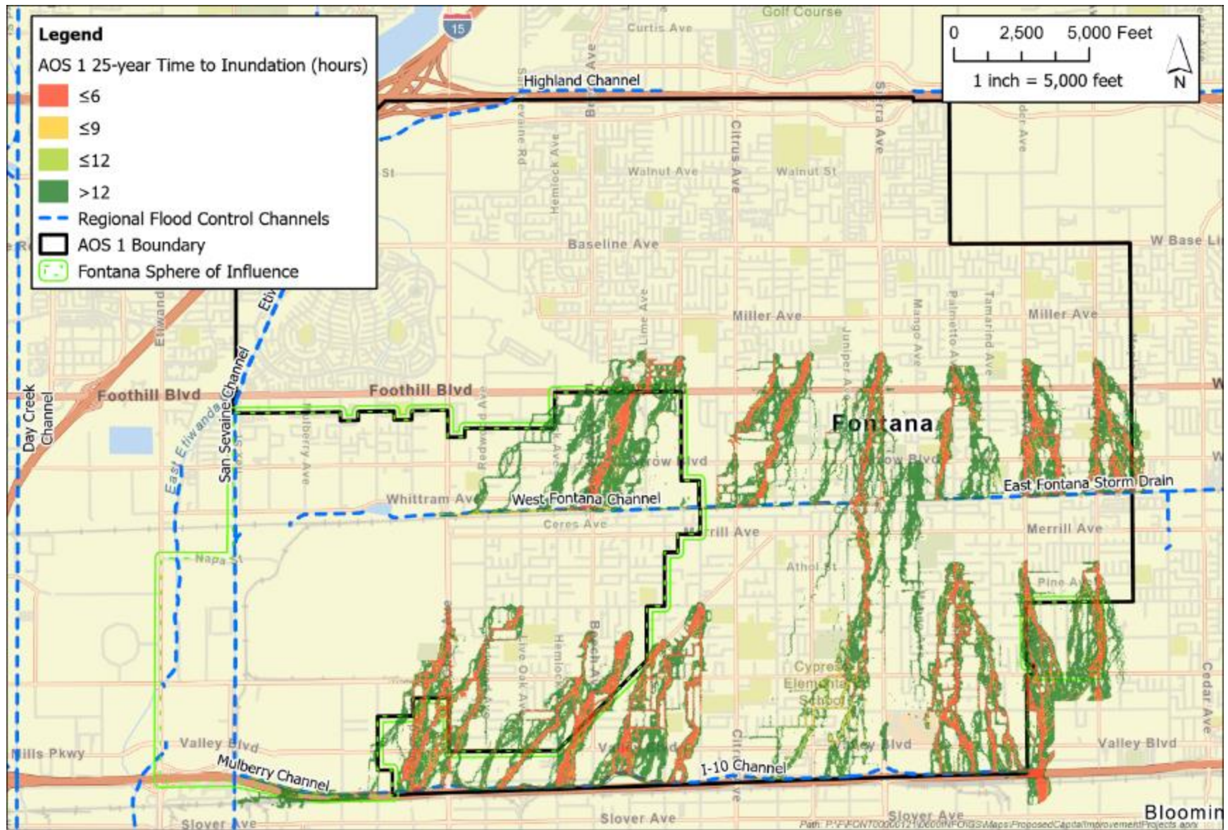
Figure 3-17. 25-year Time to Inundation for AOS 1
