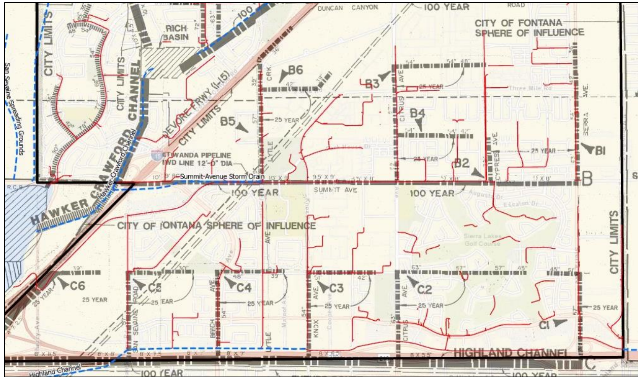
Figure 2-6. Comparison of B and C Lines from the 1992 Master Plan to Existing Pipes in AOS 3 (red lines)
