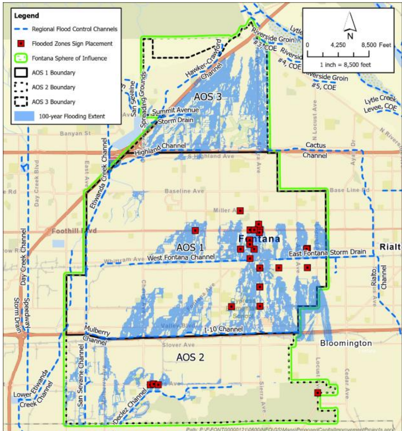
Figure 3-10. 100-year Storm Existing Conditions Hydraulic Modeling Results for Model Validation
