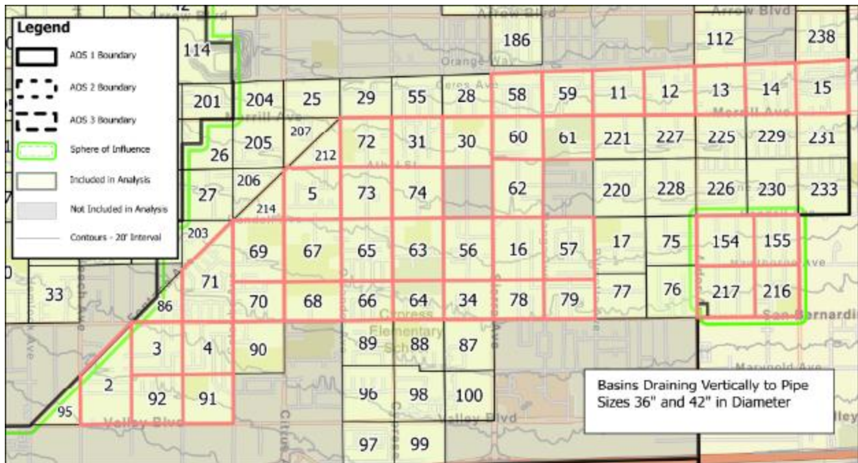
Figure 3-3. Detailed of Collector Basin Delineation for 'M' Line Portion of AOS 1 for Pipe Sizes 36" through 42".
