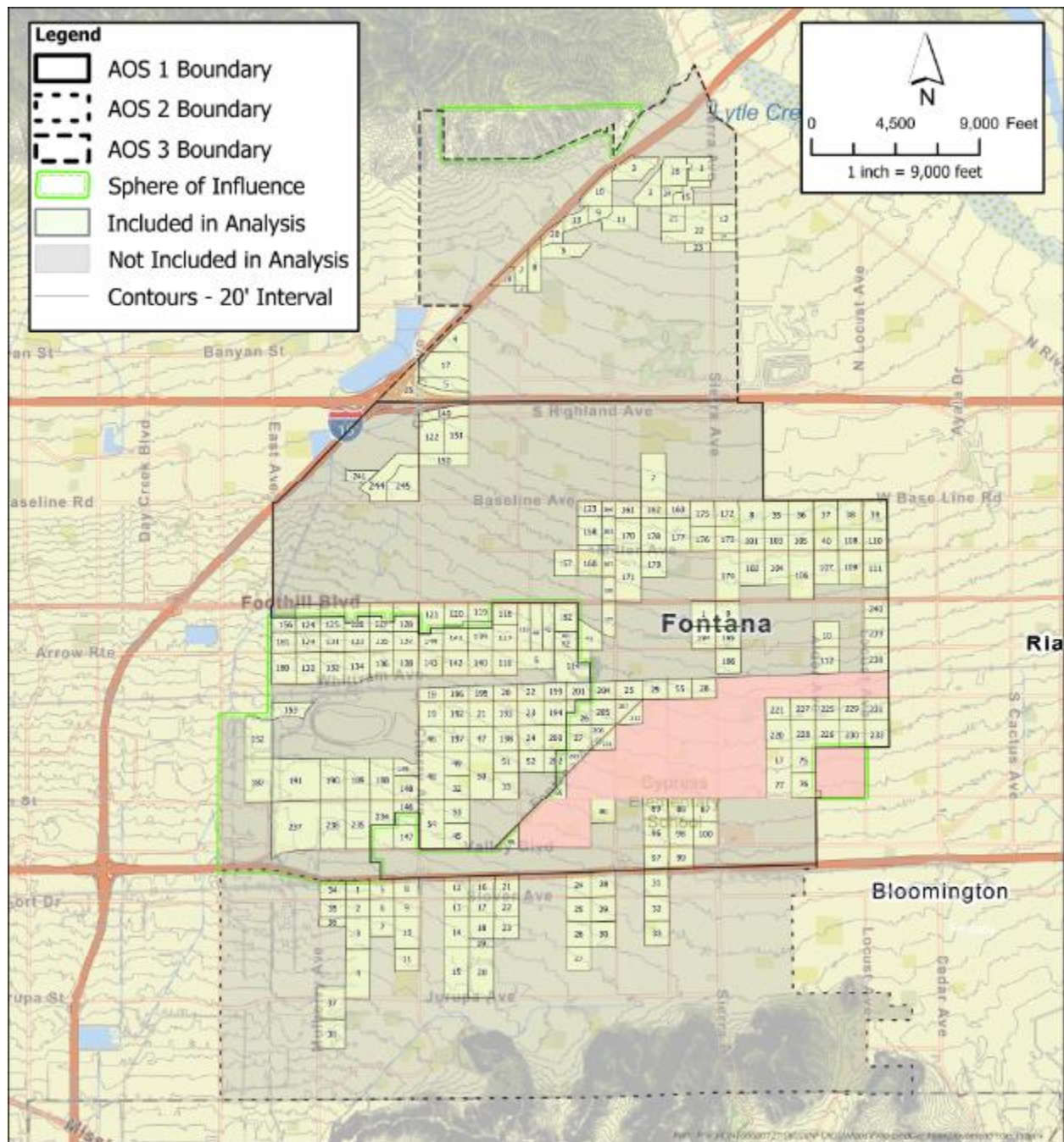
Figure 3-2. Subbasins Used in the Collector Hydrologic Analysis. Areas in Pink Shown in Detail in Figure 3-4.
