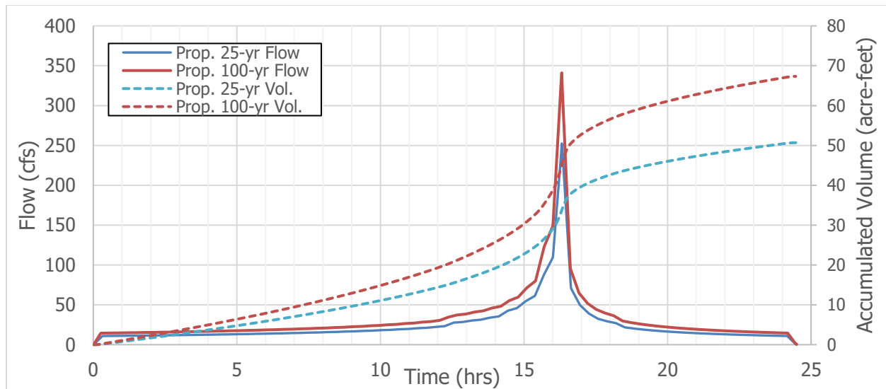
Figure 3-6. Flow and Accumulated Volume for Subbasin D7 in AOS 1 for the 25- and 100-year storms
