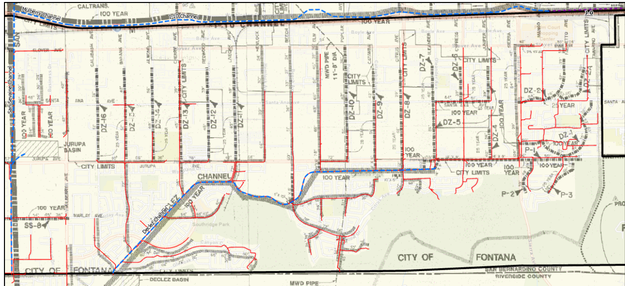
Figure 2-5. Comparison of DZ Lines from the 1992 Master Plan to Existing Pipes in AOS 2 (red lines)
