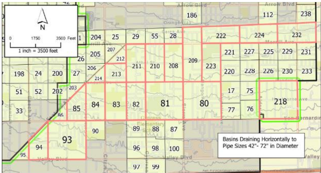
Figure 3-4. Detailed of Collector Basin Delineation for 'M' Line Portion of AOS 1 for Pipe Sizes 42" through 72"
